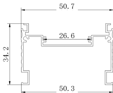
5065 tube housing
