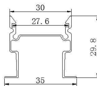
3550 tube housing
