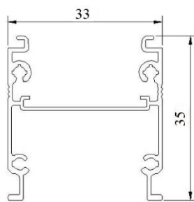
3555 tube housing
